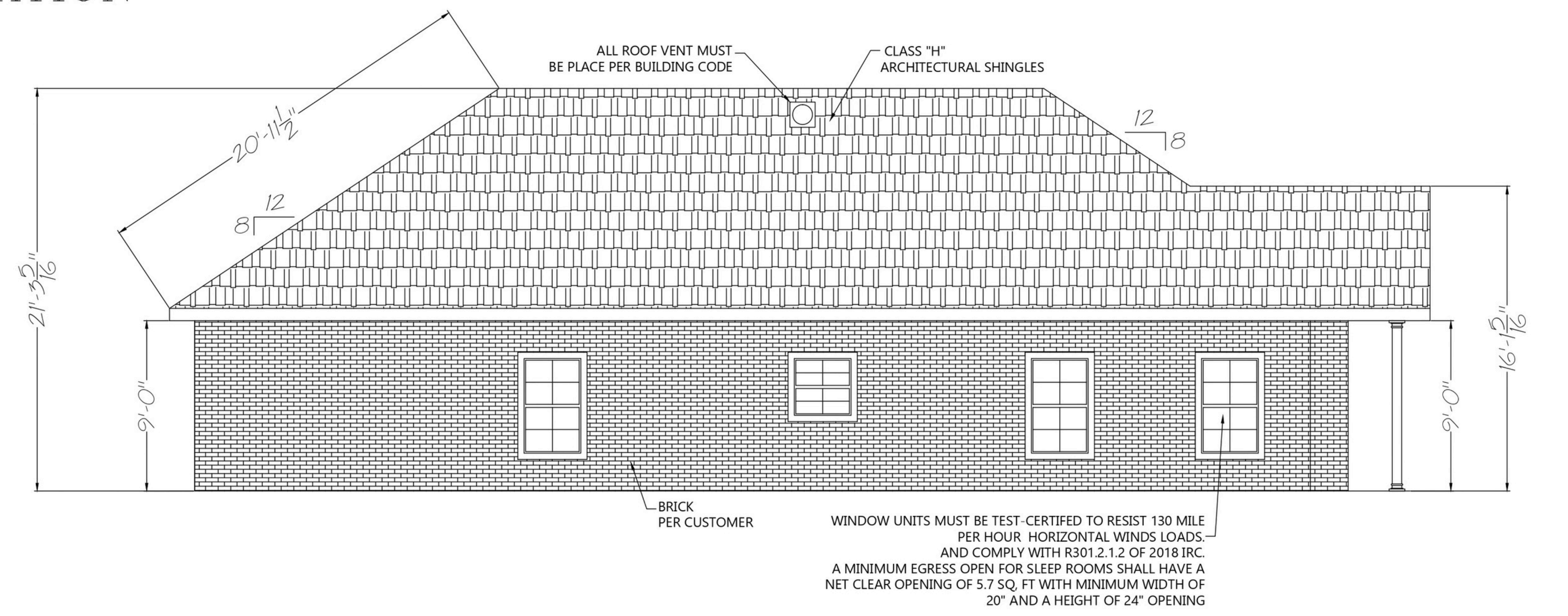
LEFT ELEVATION
